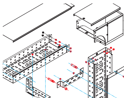
Curva in discesa 90° sghemba dx Right-hand skew outside bend 90°
