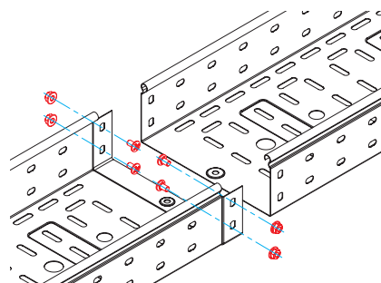
Incastro "maschio-femmina" - h 100 mm "Male-Female" snap-on joint - h 100 mm
