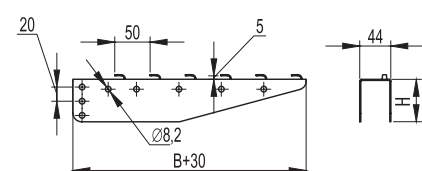
Base mensola 200-300 Base bracket 200-300
