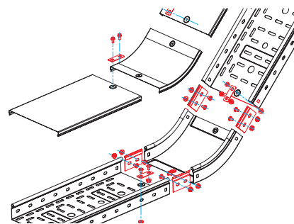
Curva in salita 45° Inside bend 45°
